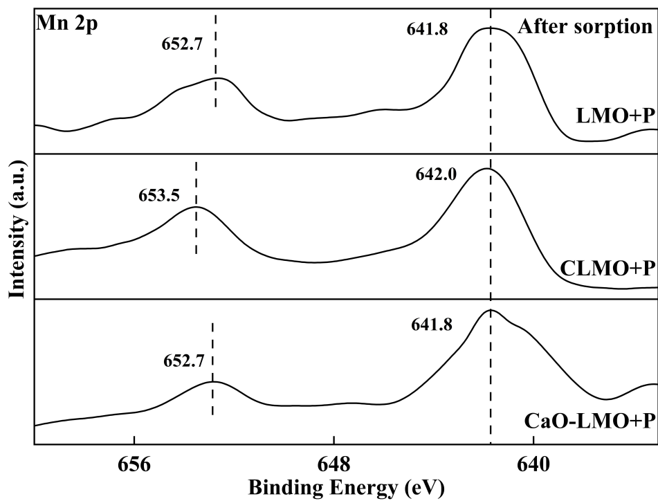
FIGURE S6. XPS of Mn 2p after phytic acid adsorption by the adsorbents
