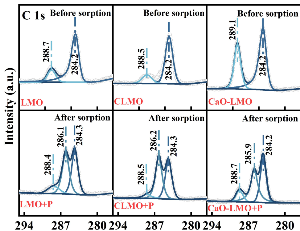
FIGURE S5. XPS of C 1s before and after phytic acid adsorption by the adsorbents.
