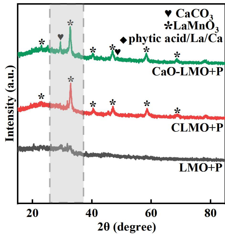
FIGURE S1. XRD patterns at 2θ diffraction angles (15°~ 85°) before and after phytic acid adsorption
