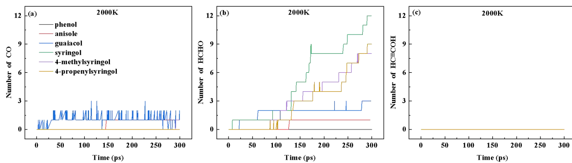
Fig. S6 Quantity-time profiles of CO, HCHO, and HC \equiv COH generated from the six model compounds at 2000 K.
