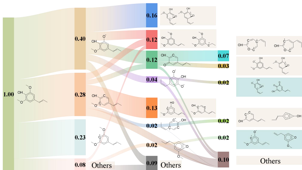
Fig. S5 Sankey diagram of the initial pyrolysis mechanisms of 4-propenylsyringol at 3500 K.
