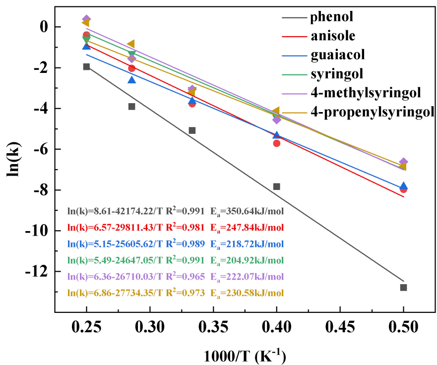
Fig. S2 Pyrolysis kinetic parameters at different temperatures.
