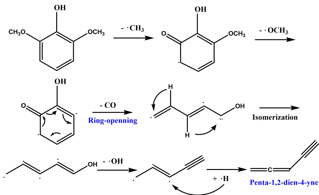
Fig. S3 Reaction pathway for C 5 H 4 formation from syringol via aromatic ring-opening.
