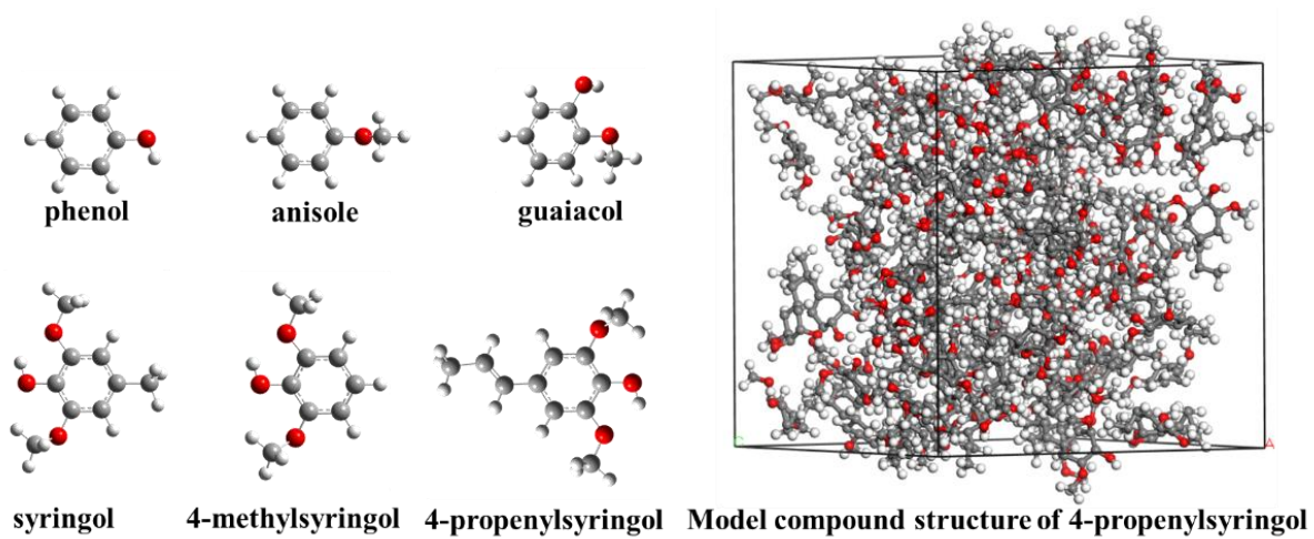
Fig. S1 Molecular structures of six lignin model monomers and a schematic of the simulation model constructed from 100 4-propenylsyringol molecules.
