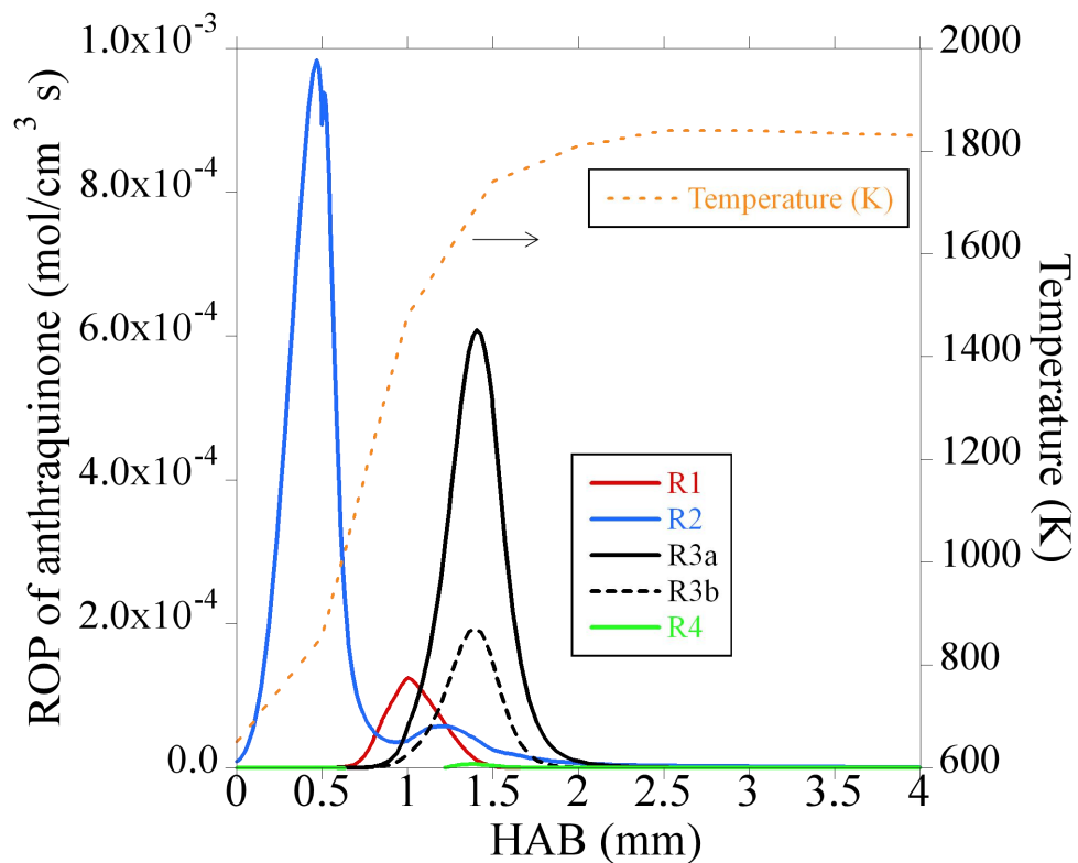
Figure S7. Analyzed ROP profiles of anthraquinone in the premixed flame of anisole. Red-solid, blue-solid, black-solid, black-dashed, green-solid, and orange-dotted lines represent R1, R2, R3a, R3b, R4, and temperature, respectively. Measured temperature data [4] for ethylbenzene premixed flame is used as input data and is shown for reference.
