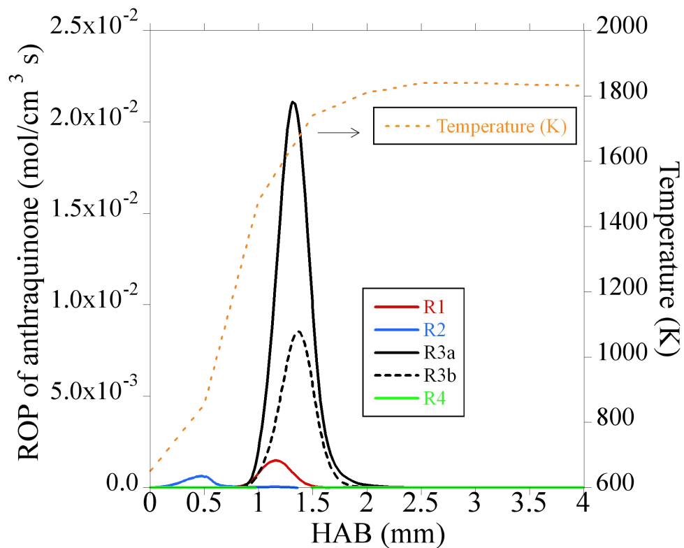
Figure S5. Analyzed ROP profiles of anthraquinone in the premixed flame of toluene. Red-solid, blue-solid, black-solid, black-dashed, green-solid, and orange-dotted lines represent R1, R2, R3a, R3b, R4, and temperature, respectively. Measured temperature data [4] for ethylbenzene premixed flame is used as input data and is shown for reference.
