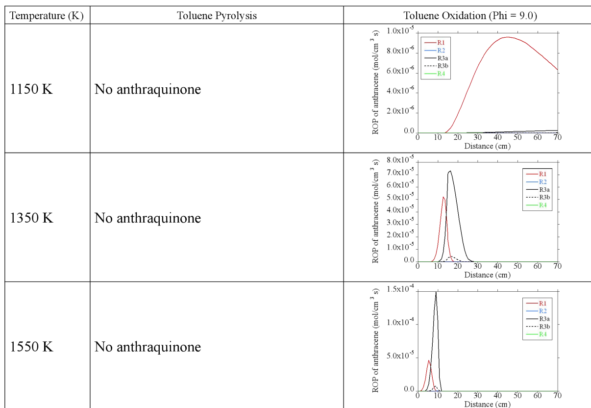
Figure S4. Analyzed ROP profiles of anthraquinone in the fuel-rich oxidation of toluene in a flow reactor at three temperatures, 1150 K, 1350 K, and 1550 K. Note that analyzed results in pyrolysis is not presented because of no anthraquinone production. Red-solid, blue-solid, black-solid, black-dashed, and green-solid lines represent R1, R2, R3a, R3b, and R4, respectively.
