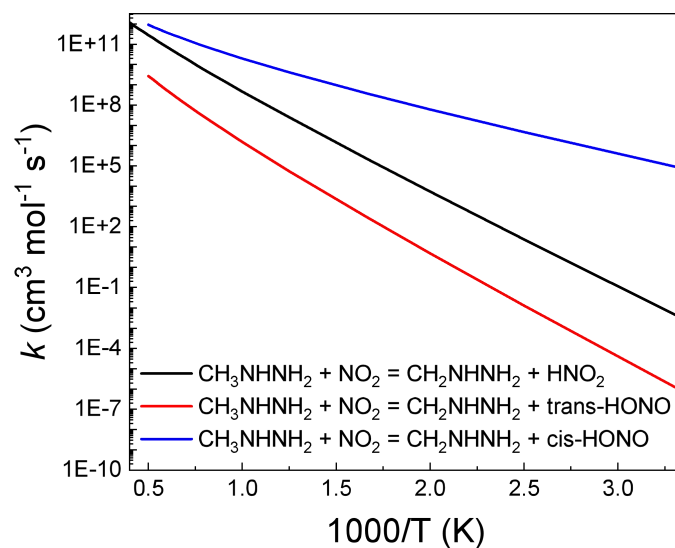
Supplementary Fig. S22 High-pressure-limit rate constants for the H-abstraction reactions of \text{CH}_3\text{NHNH}_2 on the \text{CH}_3 group with \text{NO}_2 attacking.
