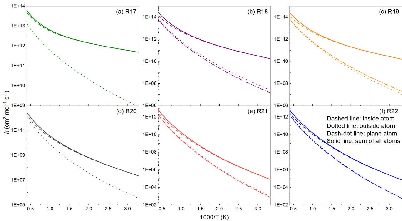
Supplementary Fig. S21 Rate constants for the H-abstraction reactions at H_{\text{inside}} , H_{\text{outside}} , and H_{\text{plane}} atoms of UDMH by H and \text{CH}_3 .
