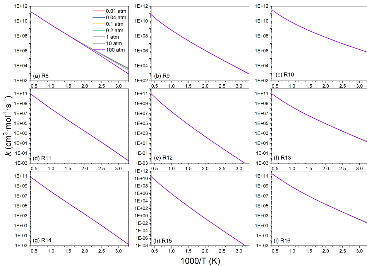
Supplementary Fig. S19 Pressure-dependent rate constants of the H-abstraction reactions of UDMH with \text{NO}_2 attacking.
