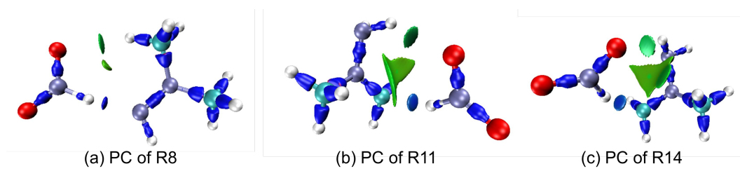
Supplementary Fig. S18 Iso-surface map of the product complex (PC) structure of (a) R8, (b) R11, and (c) R14 based on the IRI function analysis.
