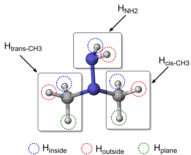
Supplementary Fig. S17 H-atom abstraction sites in UDMH.
