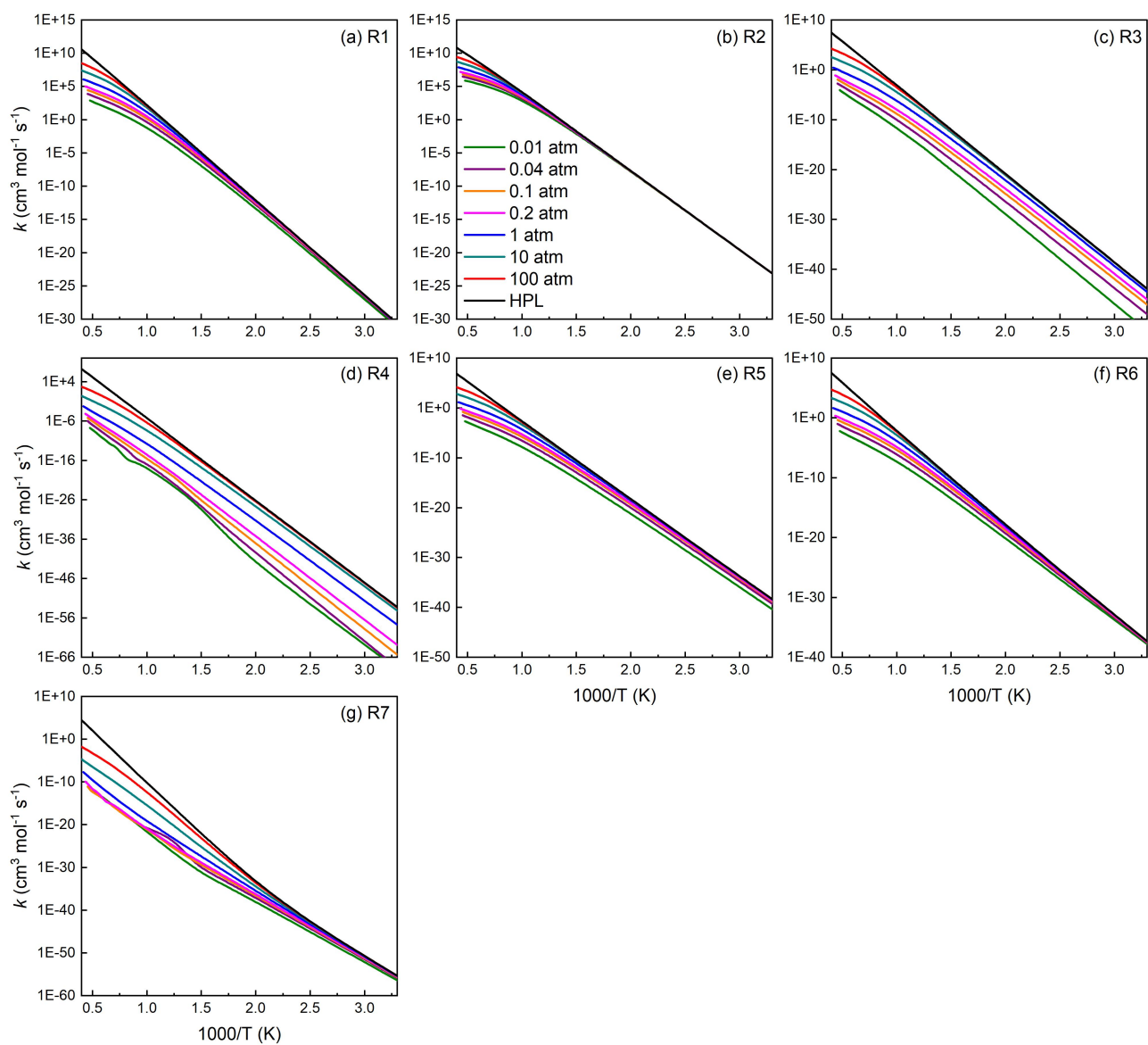
Supplementary Fig. S16 Pressure-dependent rate constants of the unimolecular decomposition reactions of UDMH.
