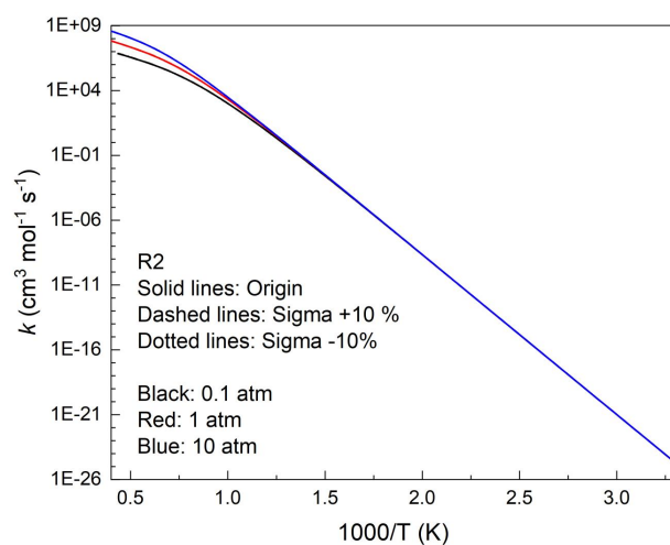
Supplementary Fig. S15 The influence of collisional parameters at 300-2500 K and 0.1-10 atm. \sigma was changed by 10% for the uncertainty analysis.
