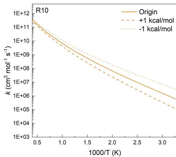
Supplementary Fig. S14 The influence of barrier heights at 300-2500 K and 100 atm. The barrier heights were changed by 1 kcal/mol for the uncertainty analysis.
