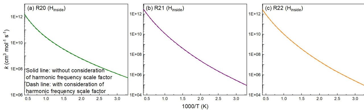
Supplementary Fig. S13 The influence of the harmonic frequency scale factor on the calculated rate constants for the H-abstraction reactions involving H_{\text{inside}} atoms by \text{CH}_3 .
