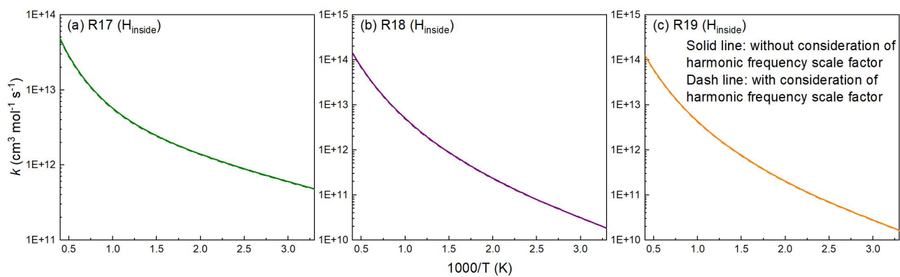
Supplementary Fig. S12 The influence of the harmonic frequency scale factor on the calculated rate constants for the H-abstraction reactions involving \text{H}_{\text{inside}} atoms by H.
