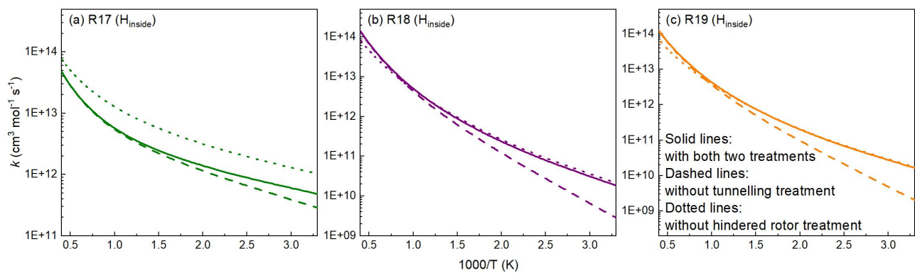
Supplementary Fig. S9 Effects of tunnelling treatment and hindered rotor treatment on the rate constants for the H-abstraction reactions involving \text{H}_{\text{inside}} atoms by H.
