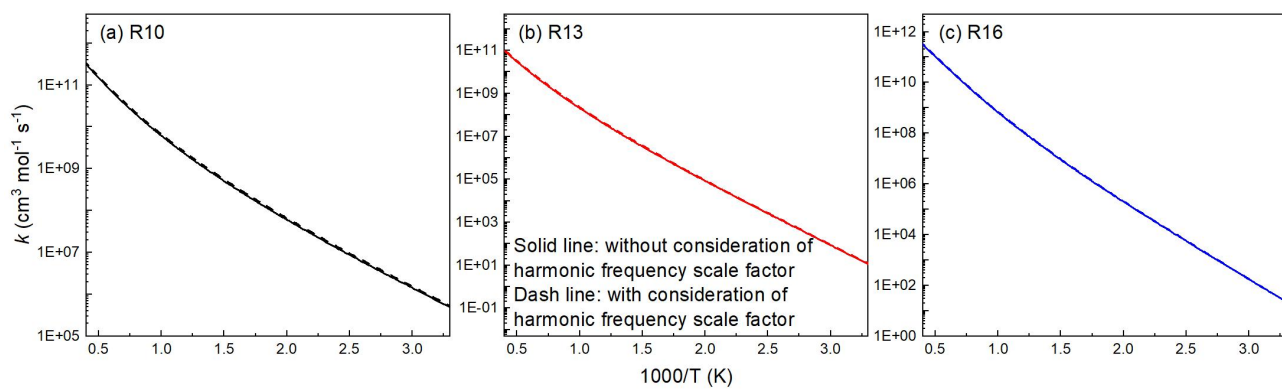
Supplementary Fig. S11 The influence of the harmonic frequency scale factor on the calculated rate constants of R10, R13, R16.
