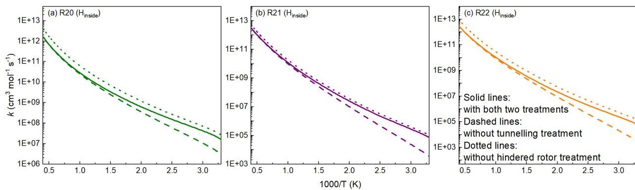
Supplementary Fig. S10 Effects of tunnelling treatment and hindered rotor treatment on the rate constants for the H-abstraction reactions involving \text{H}_{\text{inside}} atoms by \text{CH}_3 .
