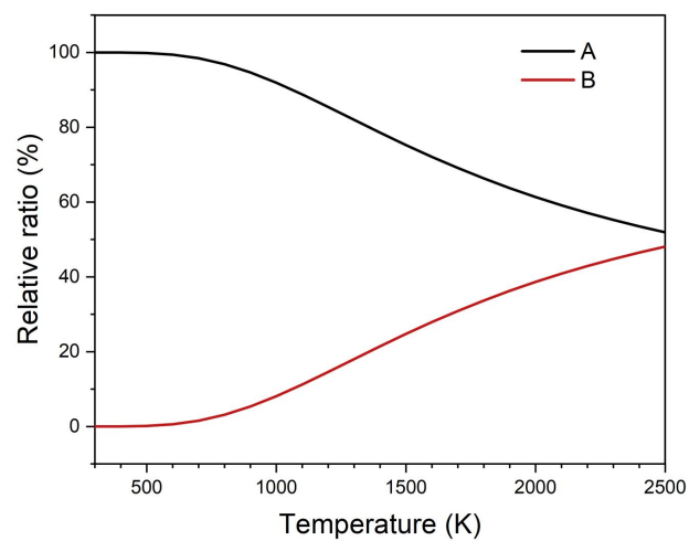
Supplementary Fig. S5 Calculated Boltzmann distributions of A and B conformers over 300-2500 K.
