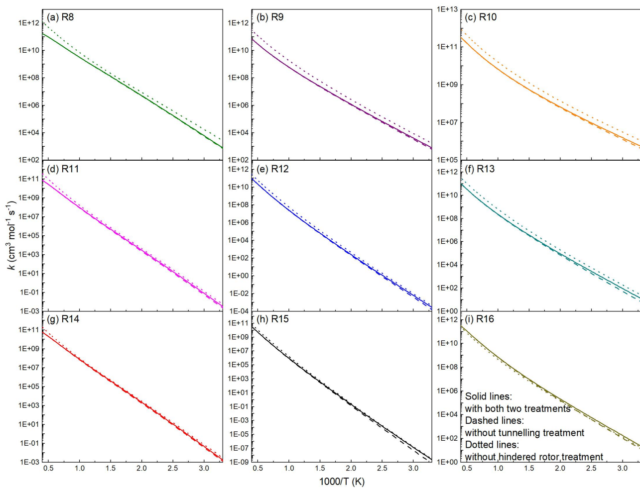
Supplementary Fig. S8 Effects of tunnelling treatment and hindered rotor treatment on the rate constants for R8-R16.
