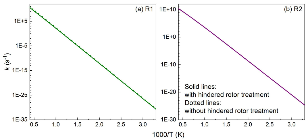
Supplementary Fig. S7 Effects of hindered rotor treatment on the rate constants for R1 and R2.
