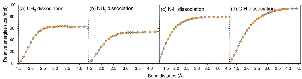
Supplementary Fig. S6 The calculated MEP results for the unimolecular bond dissociation reactions of UDMH.
