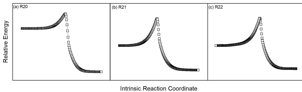
Supplementary Fig. S4 IRC results for the H-abstraction reactions of UDMH with CH 3 attacking.
