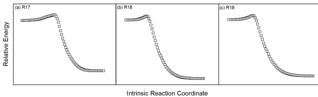
Supplementary Fig. S3 IRC results for the H-abstraction reactions of UDMH with H attacking.
