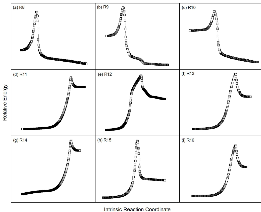
Supplementary Fig. S2 IRC results for the H-abstraction reactions of UDMH with NO 2 attacking.
