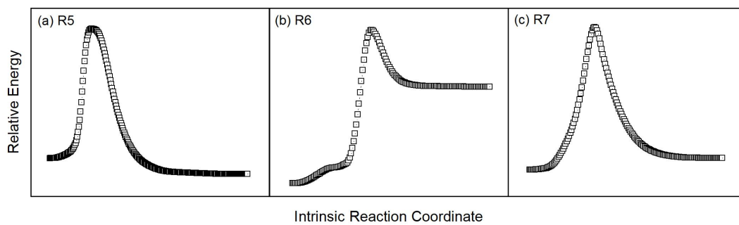
Supplementary Fig. S1 IRC results for the elimination reactions of UDMH.
