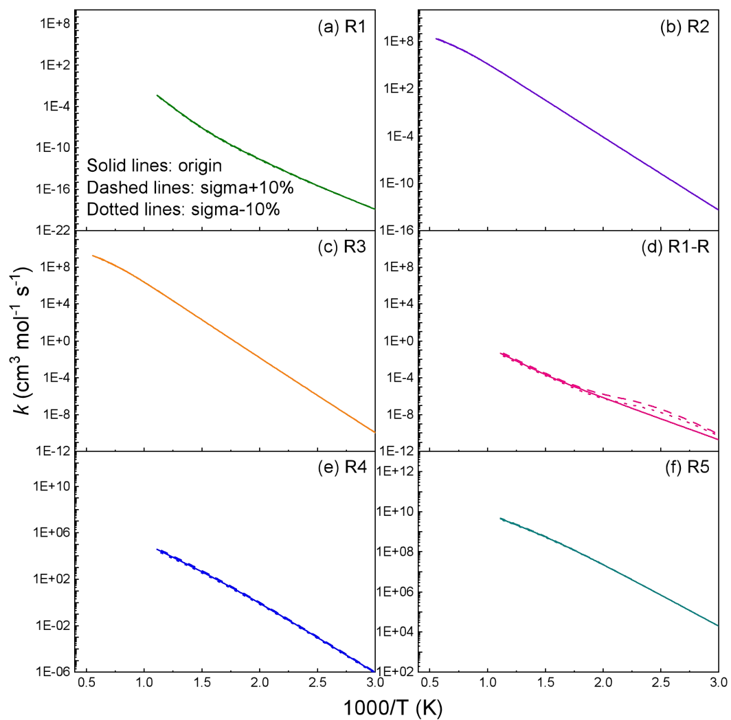
Supplementary Fig. S6 The influence of collisional parameters changing on the rate constants of R1-R5 at 300-2500 K and 100 atm. \sigma was changed by 10% for the uncertainty analysis.
