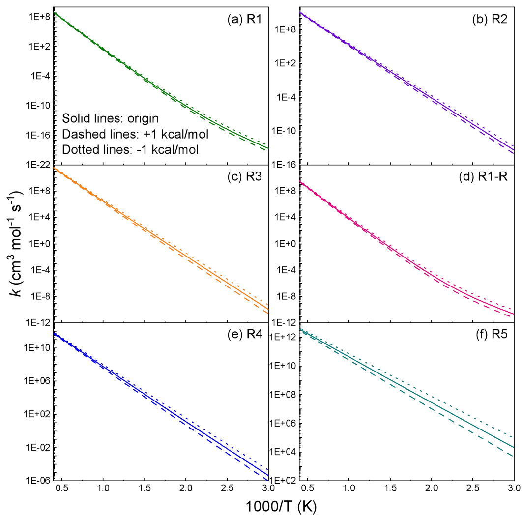
Supplementary Fig. S5 The influence of energy barrier changing on the rate constants of R1-R5 at 300-2500 K and 100 atm. The energy barriers were changed by 1 kcal/mol for the uncertainty analysis.
