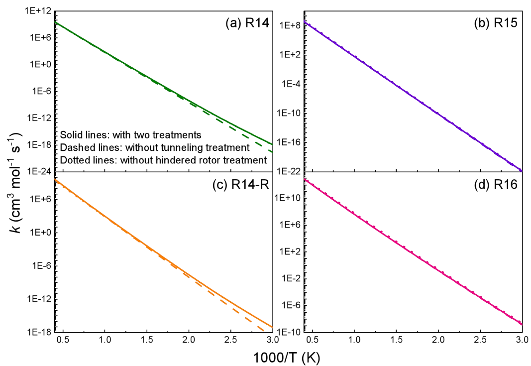
Supplementary Fig. S4 Effects of tunnelling treatment and hindered rotor treatment on the rate constants of R14-R16 and R14-R.
