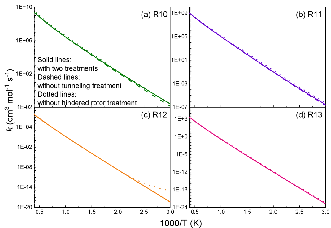
Supplementary Fig. S3 Effects of tunnelling treatment and hindered rotor treatment on the rate constants of R10-R13.
