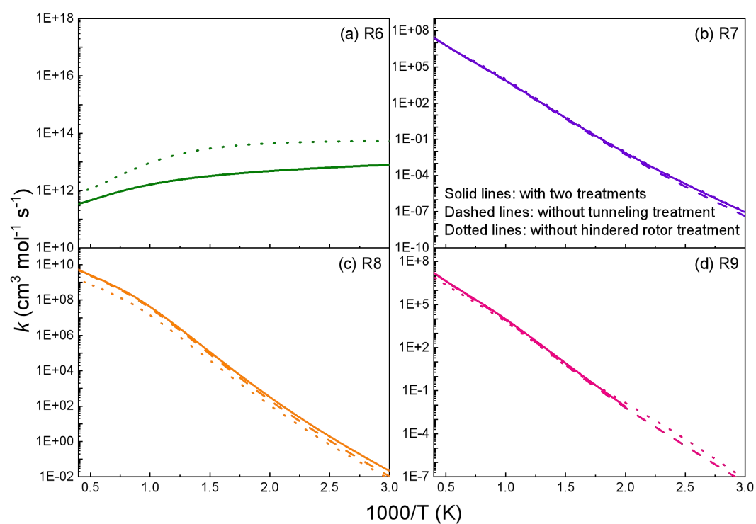
Supplementary Fig. S2 Effects of tunnelling treatment and hindered rotor treatment on the rate constants of R6-R9.
