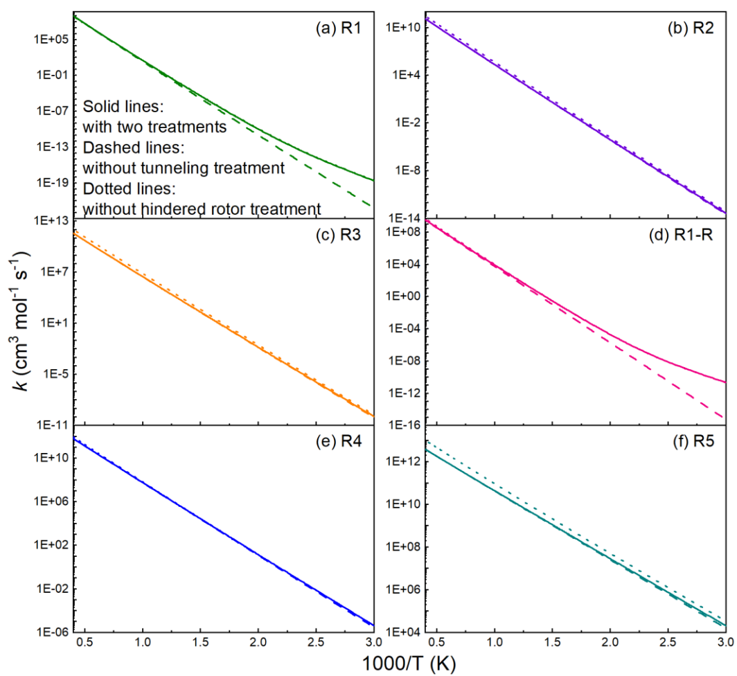
Supplementary Fig. S1 Effects of tunnelling treatment and hindered rotor treatment treatment on the rate constants of R1-R5 and R1-R.
