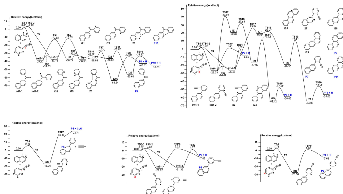
Fig. S2. Potential energy profiles for recombination reactions between 2-naphthyl and phenylacetylene at alpha-, 1-, 2-, 3-, and 4-sites.
