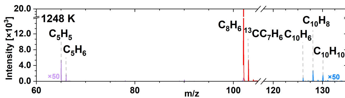
Fig. S3. Mass spectrum of the 2-naphthyl/phenylacetylene reaction in the range of m/z = 60 -135 at 1248 K, recorded at a photoionization energy of 9.5eV. Weak ion peaks (purple and blue) are multiplied by a factor of 50 for clarity.
