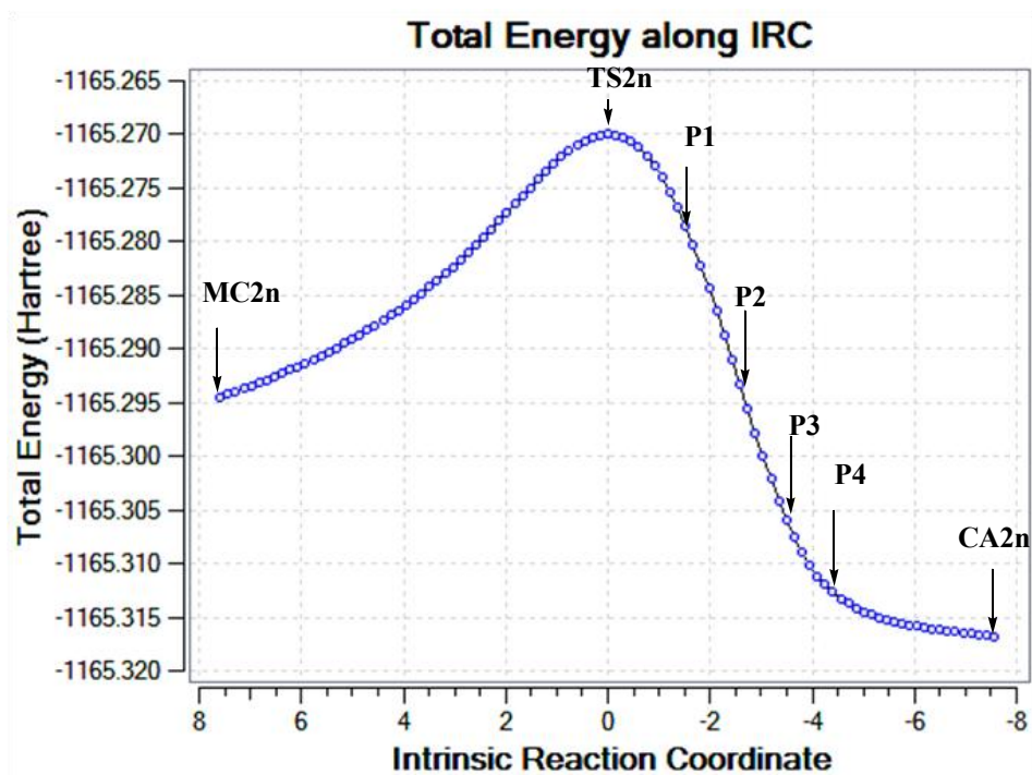
Supplementary Fig. S1. The IRC profile of the favourable TS2n together with the position of the selected points of the I32CA reaction of 1 .
