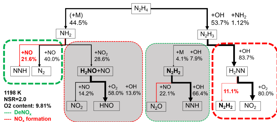
Fig. S3. The rate of product (ROP) analysis of the N 2 H 4 /NO/O 2 at [NO] initial = 450 ppm, NSR = 2.0, O 2 content = 9.81% at T = 1198 K, P = 1.0 atm, τ = 0.3 s.
