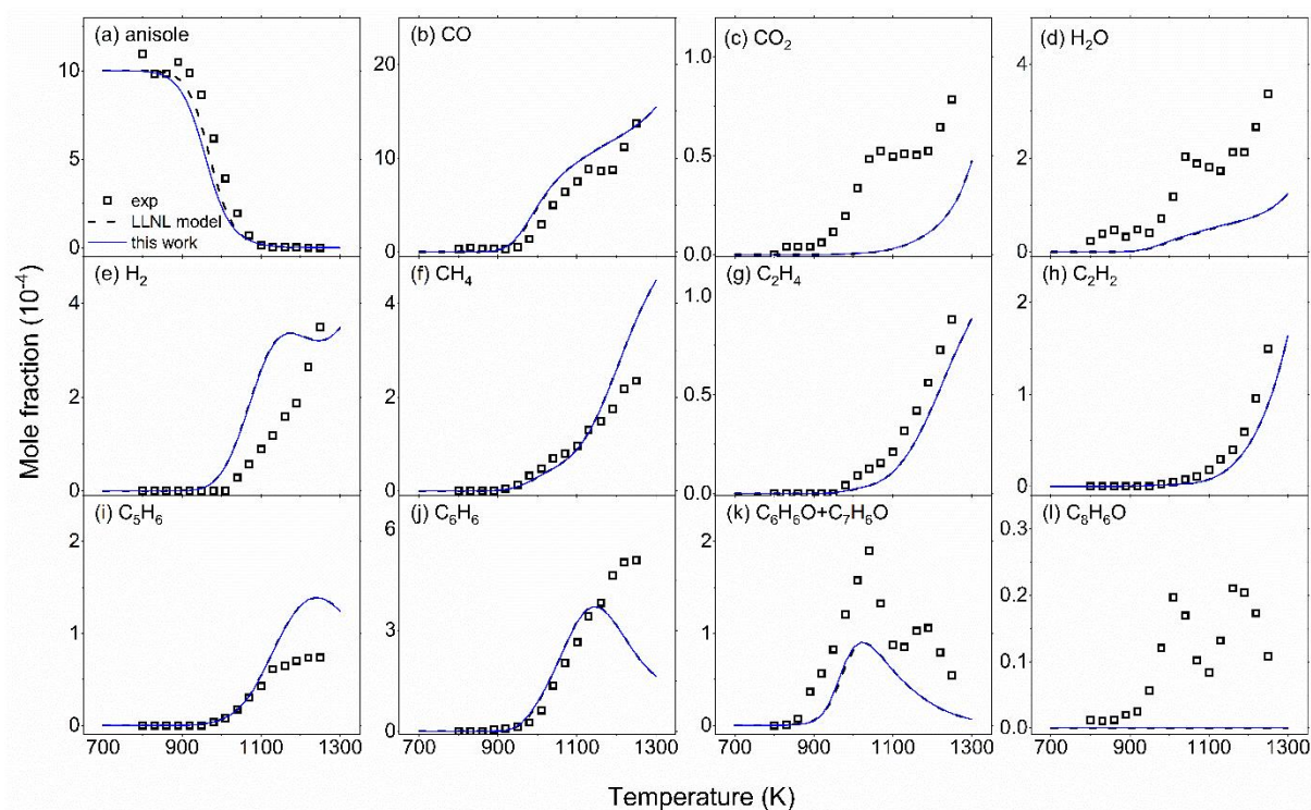
Supplementary Fig. S7. Mole fraction profiles of reactants, main products, and important intermediate species of anisole oxidation ( \phi = 2.0 ) in jet stirred reactor. Experimental data are taken from Wagnon et al. [2]. The solid lines are simulation using kinetic model developed in this work, compare to the dashed lines using LLNL model [2].
