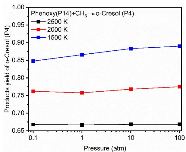
Supplementary Fig. S2. Pressure dependence of o-cresol formation from methyl radical addition to phenoxy radical.
