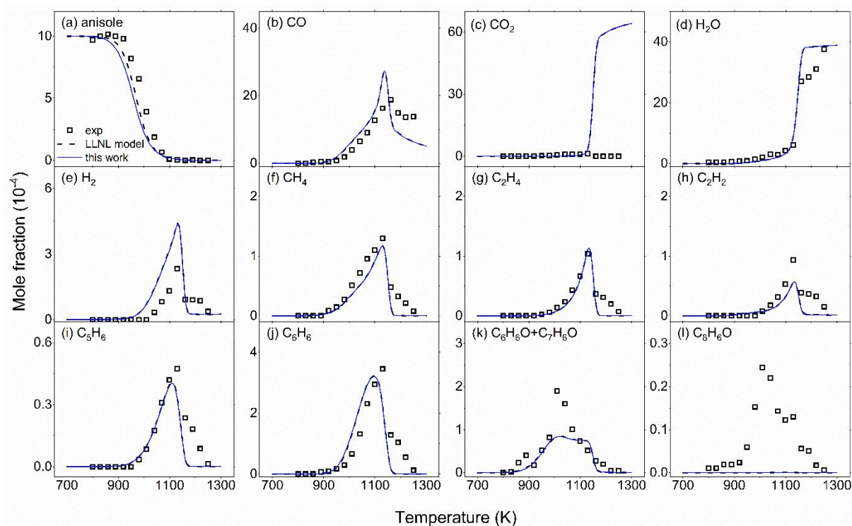
Supplementary Fig. S5. Mole fraction profiles of reactants, main products, and important intermediate species of anisole oxidation ( \phi = 0.5 ) in jet stirred reactor. Experimental data are taken from Wagnon et al. [2]. The solid lines are simulation using kinetic model developed in this work, compare to the dashed lines using LLNL model [2].
