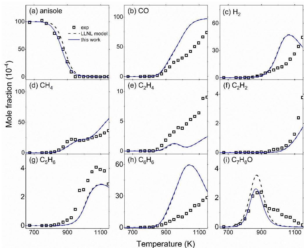
Supplementary Fig. S3. Mole fraction profiles of reactants, main products, and important intermediate species of anisole pyrolysis in jet stirred reactor. Experimental data are taken from Nowakowska et al. [1] . The solid lines are simulation using kinetic model developed in this work, compare to the dashed lines using LLNL model [2] .
