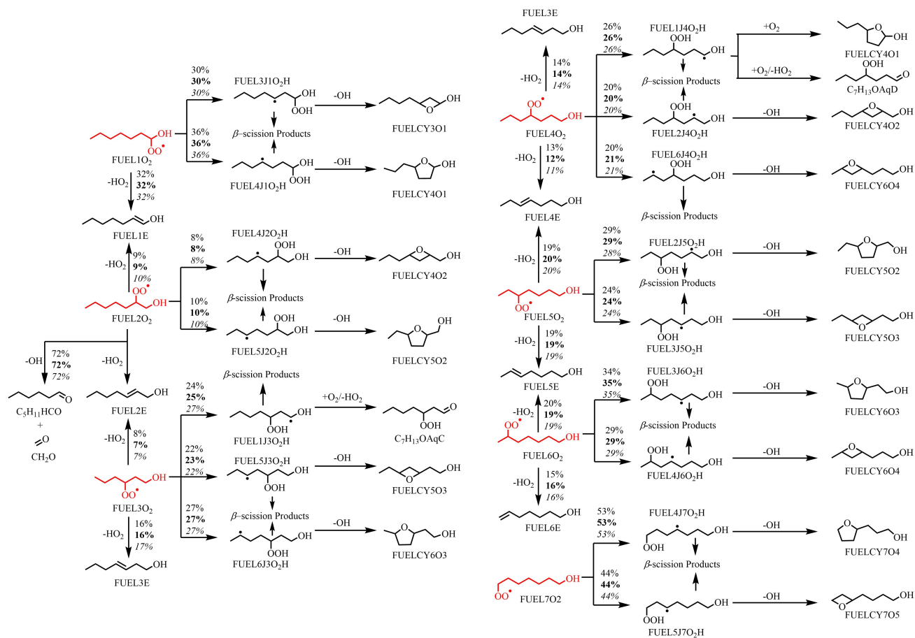
Fig S8 Rate of production (ROP) analysis for FUEL1O 2 - FUEL7O 2 at T = 790 K at atmospheric pressure and \phi = 0.5 (regular), 1.0 ( bold ), and 2.0 ( italic ). The numbers reflect the percentages of corresponding pathways in relative reaction flux.
