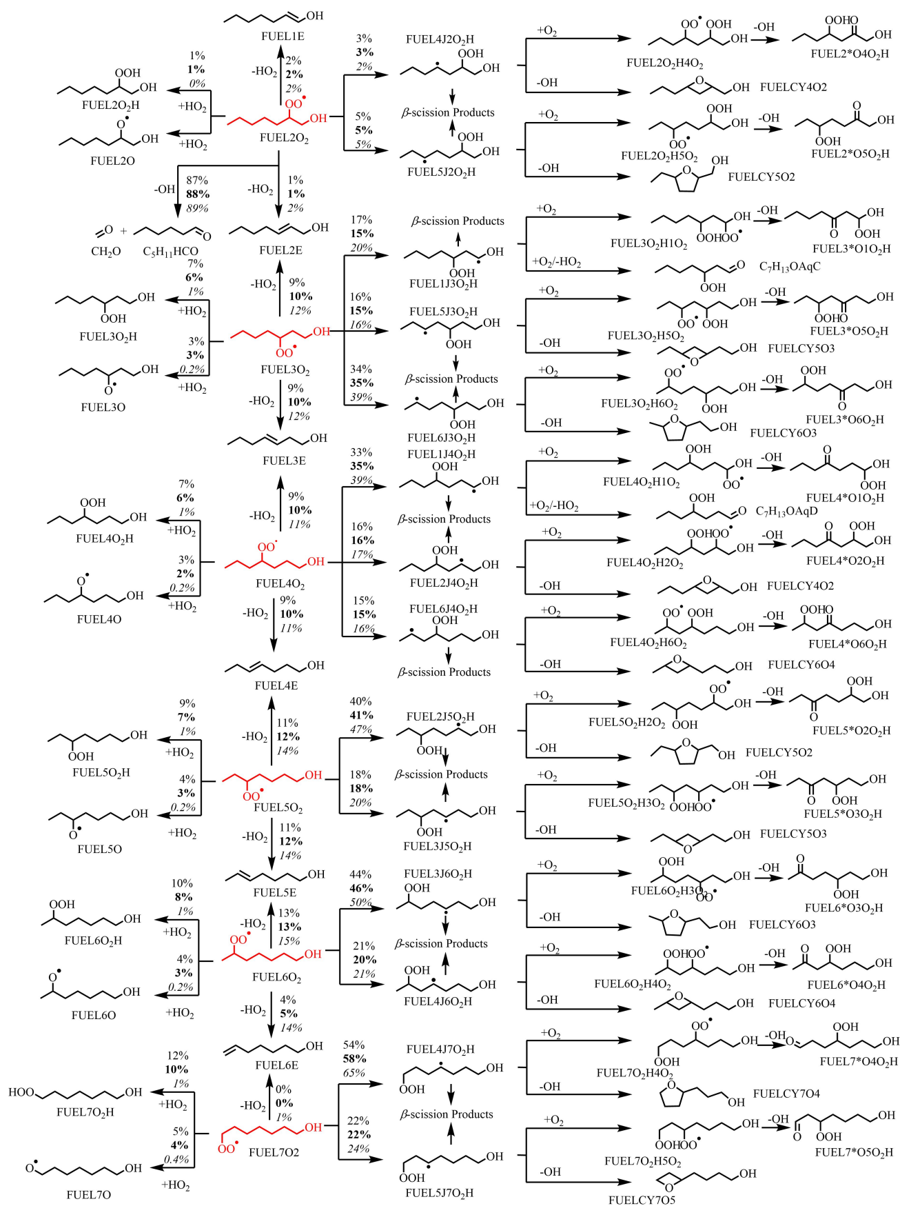
Fig S7 Rate of production (ROP) analysis for FUEL2O 2 - FUEL7O 2 at T = 610 K at atmospheric pressure and \phi = 0.5 (regular), 1.0 ( bold ), and 2.0 ( italic ). The numbers reflect the percentages of corresponding pathways in relative reaction flux.
