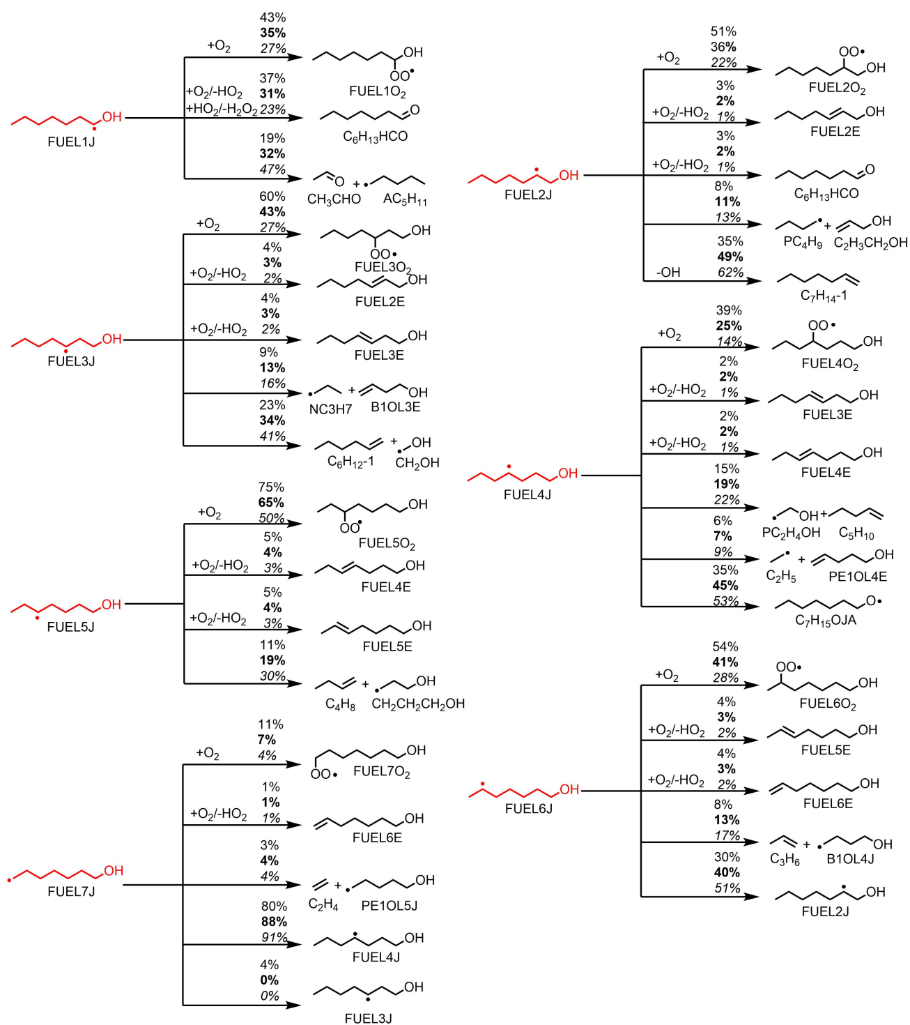
Fig. S6 Rate of production (ROP) analysis for FUEL1J - FUEL7J radicals at T = 790 K at atmospheric pressure and \phi = 0.5 (regular), 1.0 ( bold ), and 2.0 ( italic ). The numbers reflect the percentages of corresponding pathways in relative reaction flux.
