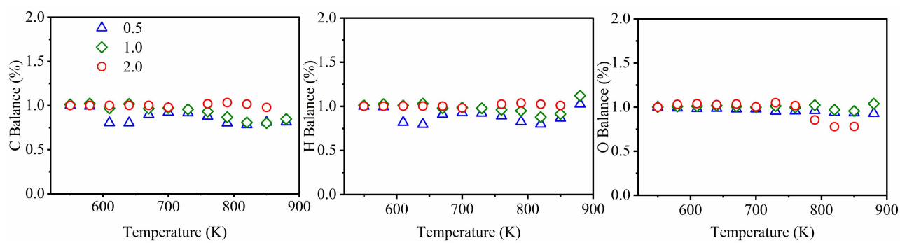
Fig. S3 C, H, and O elemental balances for n -heptanol oxidation.
